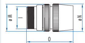
Square panel connector / Cable connector assembly
