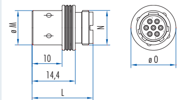
Coupler connector
