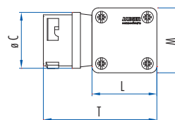
Coupler connector
