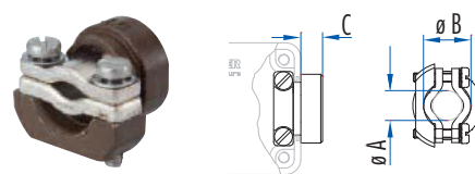
Type 3 High-Performance
