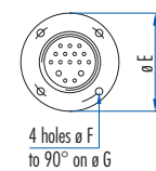
Circular male panel connectors housings 3 to 5
