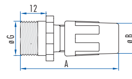
Coupler connector
