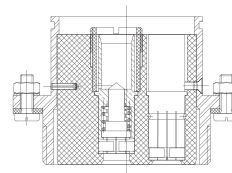
Panel connector
