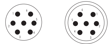
Housing 1 4 x \varnothing 2,4 mm
