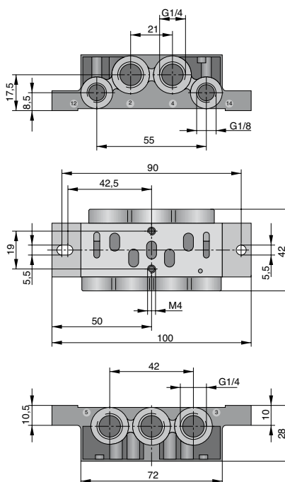
Single Base Plates Form A – Connection size G1/4 – Type: S20-01-1/4-A
